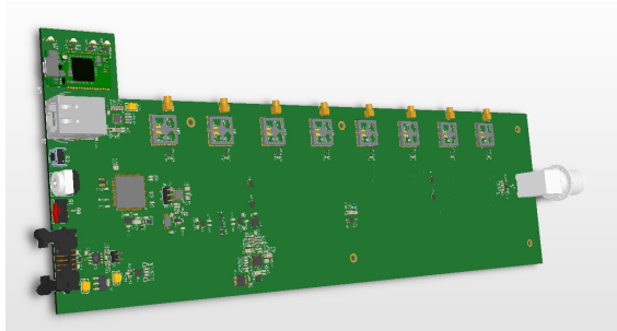
VT-RSD-5 RF Switch Detector
